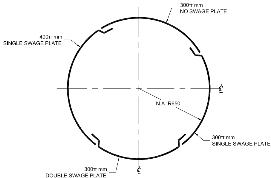
TUNNEL LINER PLATE SECTIONS
