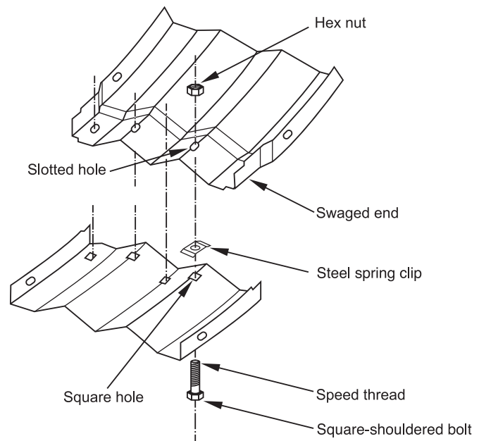
FIGURE 3: Bolting configuration
