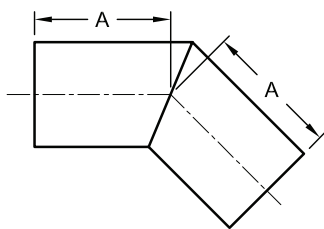
2 Piece Elbow 5° to 45°
