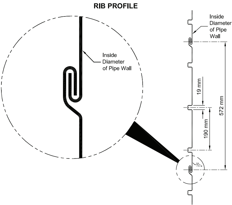
ULTRA FLO'S EXTERIOR BOX RIBS AND SMOOTH INTERIOR COMBINES STRENGTH WITH SUPERIOR HYDRAULIC PERFORMANCE
