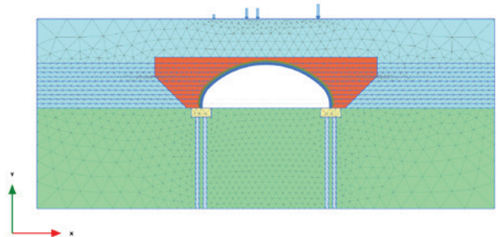
ARMTEC'S FINITE ELEMENT ANALYSIS FOR BRIDGE-PLATE DESIGN
