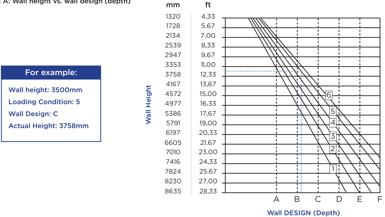
Chart A: Wall height vs. wall design (depth)
