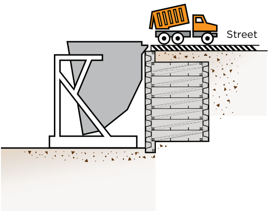
Construction of waste transfer station
